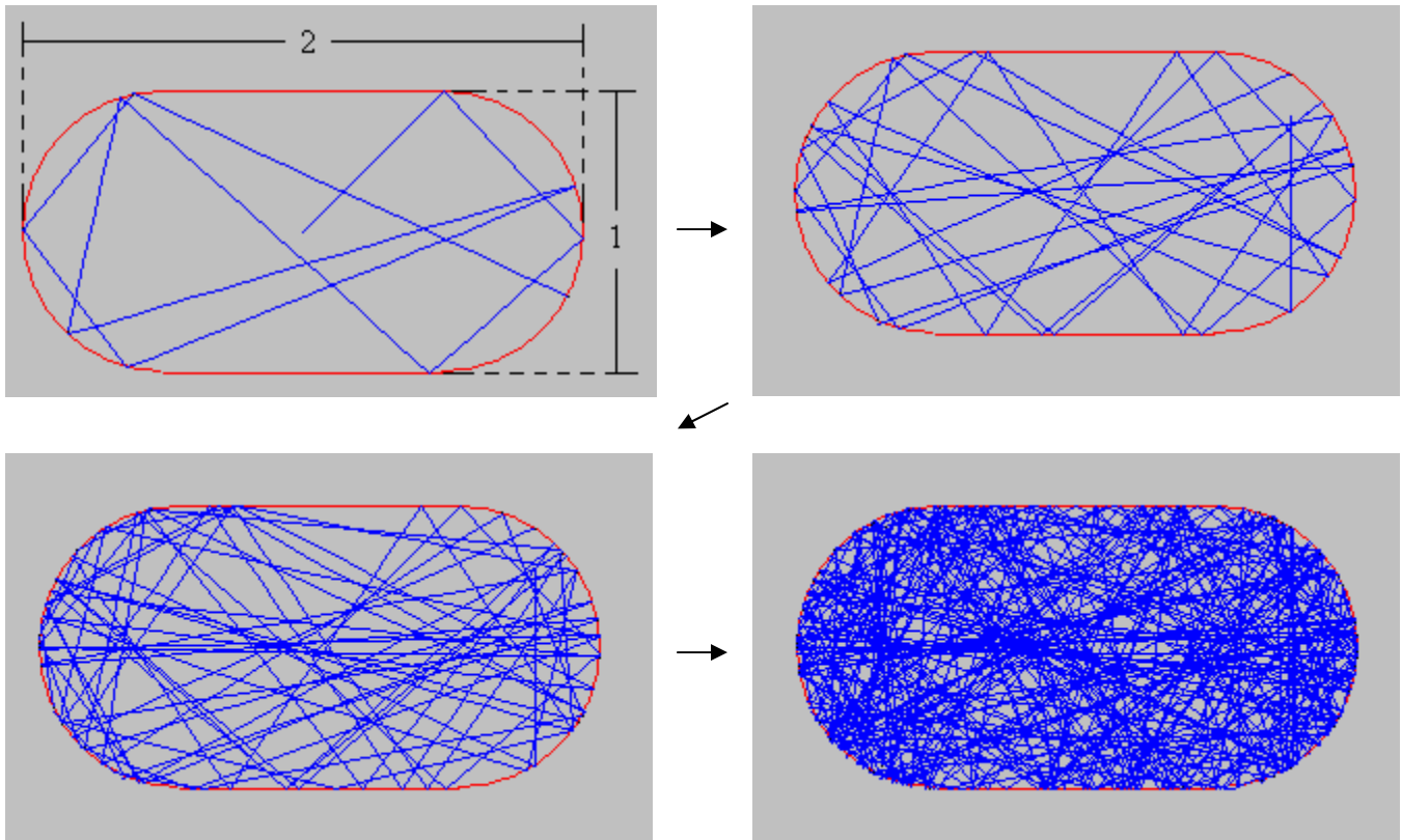
Figure 2: Stadium Billiard Problem
